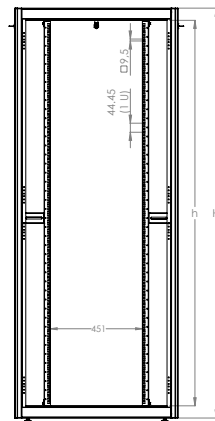
DIMENSIONS IN WIDTH AND HEIGHT
