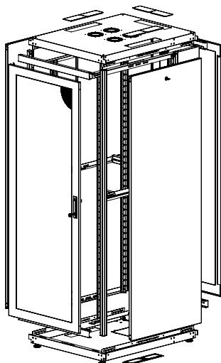
EXPLODED VIEW
