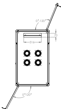
FRONT AND REAR DOOR OPENING ANGLE
