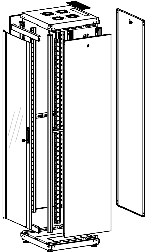
EXPLODED VIEW
