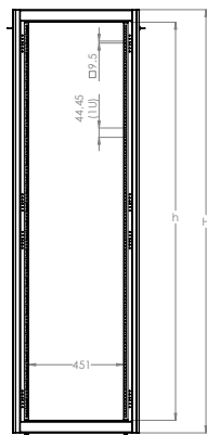
DIMENSIONS IN WIDTH AND HEIGHT
