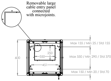
MAX/STD/MIN EQUIPMENT MOUNTING DISTANCE
