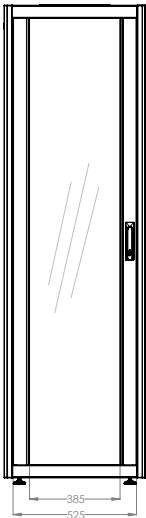
FRONT VIEW
