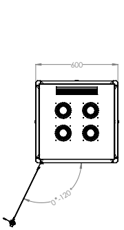
FRONT DOOR OPENING ANGLE
