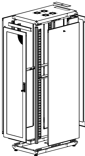
EXPLODED VIEW
