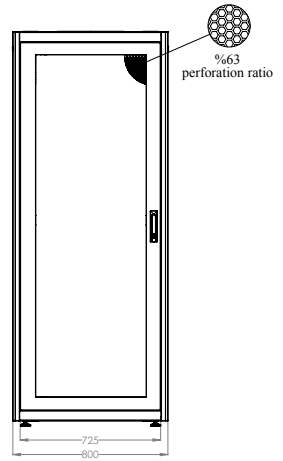
REAR VIEW
