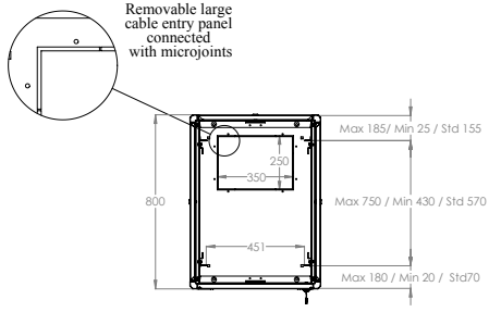
MAX / STD / MIN EQUIPMENT MOUNTING DISTANCE
