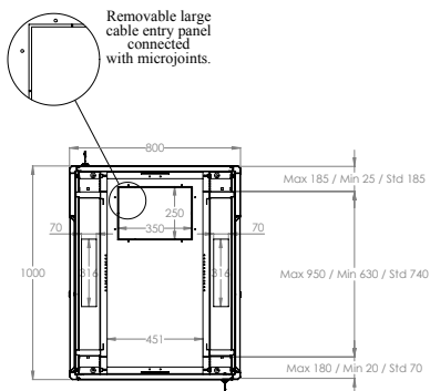
MAX/STD/MIN EQUIPMENT MOUNTING DISTANCE
