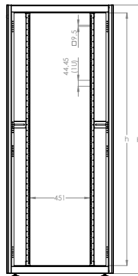
DIMENSIONS IN WIDTH AND HEIGHT
